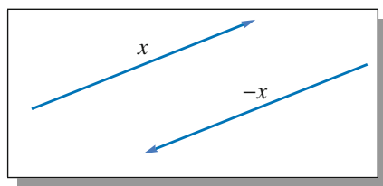
A vector and its additive inverse.
