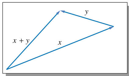
The sum of two vectors.
