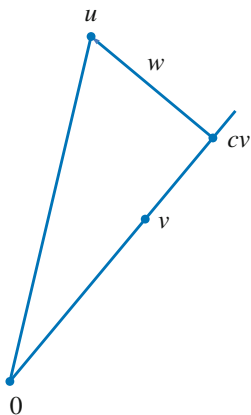
An orthogonal decomposition.
