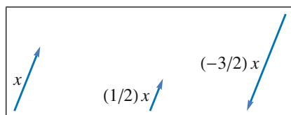
Scalar multiplication.
