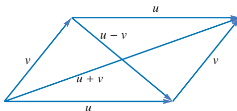
The parallelogram equality.
